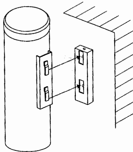
2nd step: Put the smoking post to the wall-mounted unit
