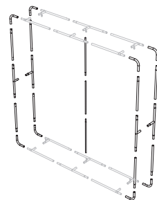
Tube Packing Bag ② Side & Center Tubes Curved Corner Tubes
